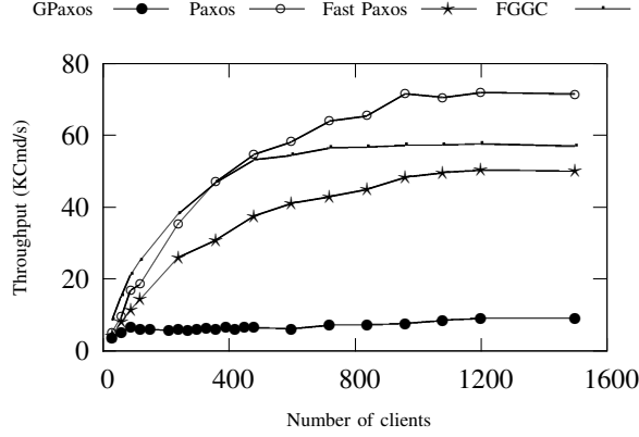
Figure 1. LAN performance
